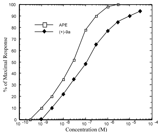
Figure 2. □ Dose–response curve of reference agonist arecaidine propargyl ester (APE); ◆ dose–response curve of agonist (+)- 9a on guinea pig ileum ( M_3 ). Each point is the mean of at least six independent observations. The SEMs are less than 10% and are not shown.
