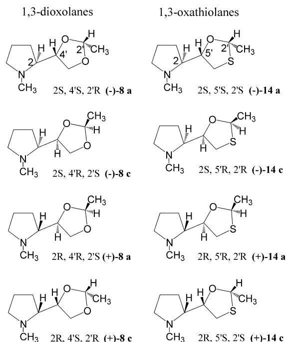
Chart 2. Absolute configuration of the obtained stereoisomers of 8 and 14 .
