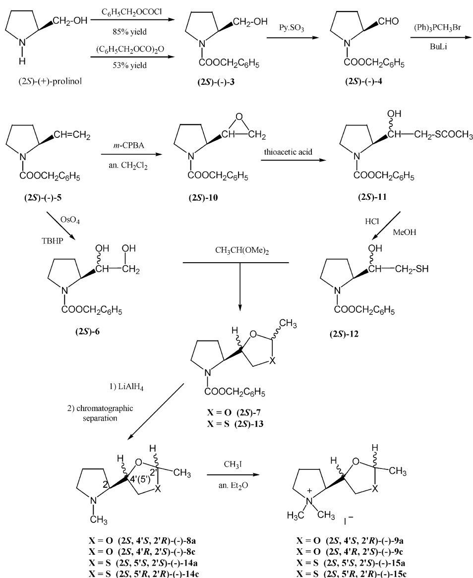
Scheme 1. (a) The same reactions were performed also on the (2R)-(-)-prolinol (not shown).
