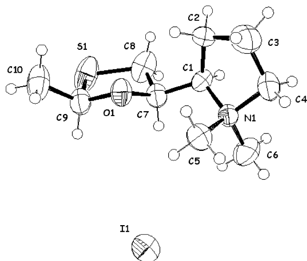
Figure 1. ORTEP drawing of compound (+)- 15a showing one of the four independent molecules in the asymmetric unit.
